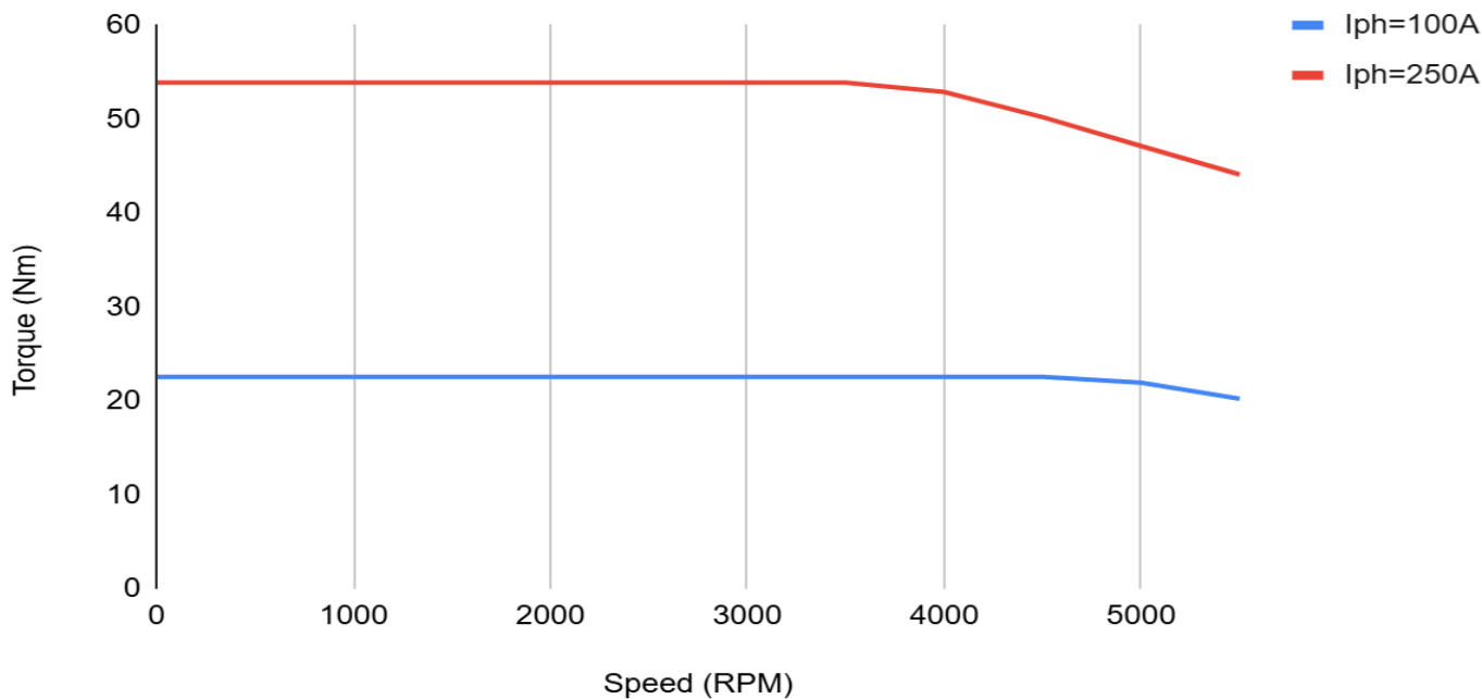
Torque vs Speed(96V)
