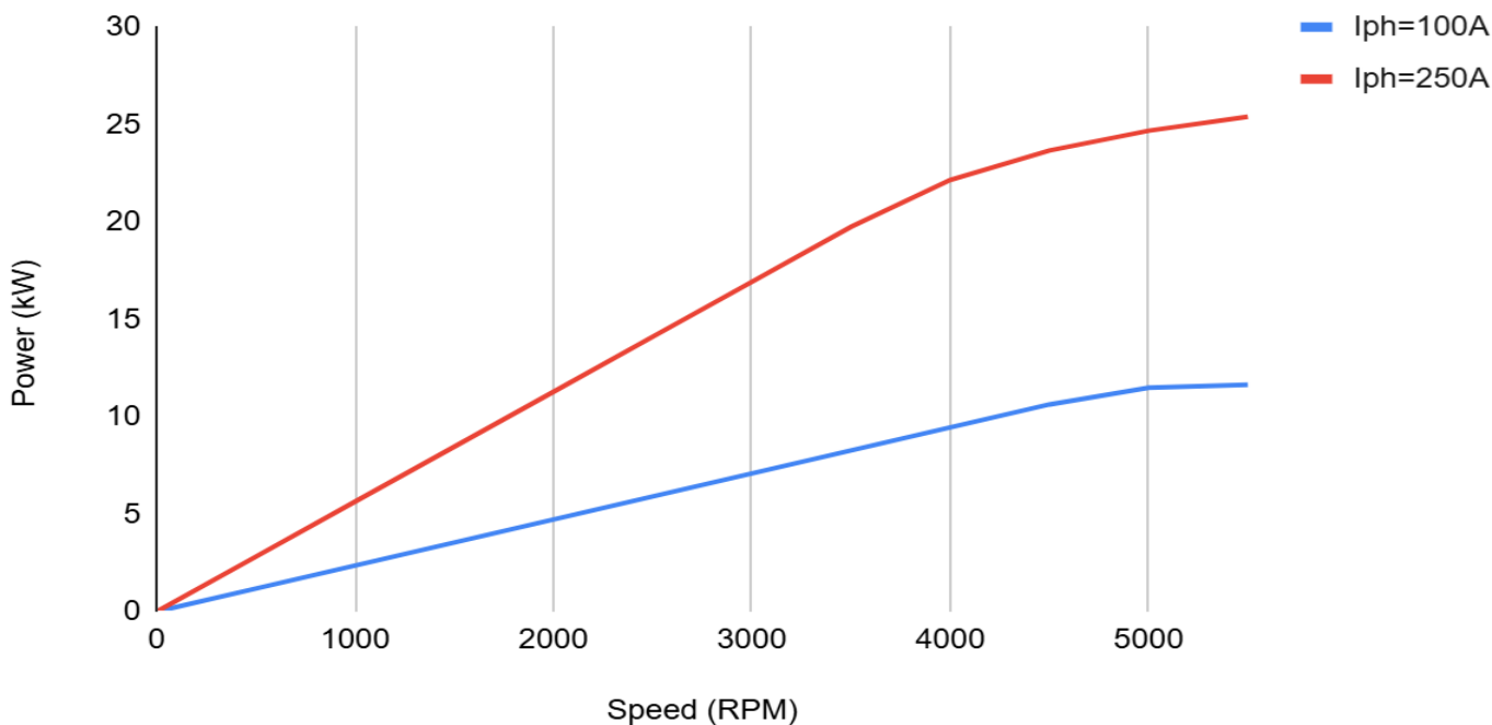
Power vs Speed(96V)
